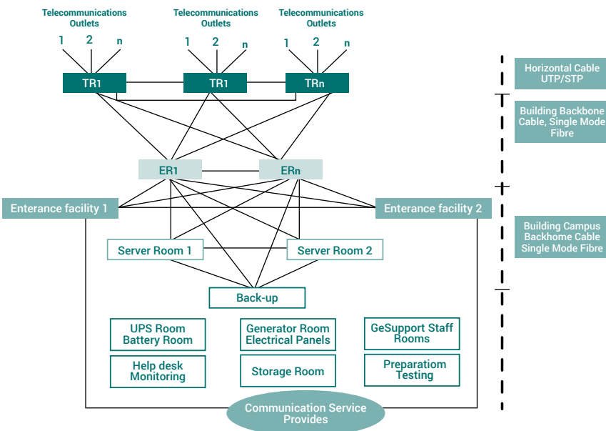
Figure 1 :Schematic Diagram for the different types of Rooms
